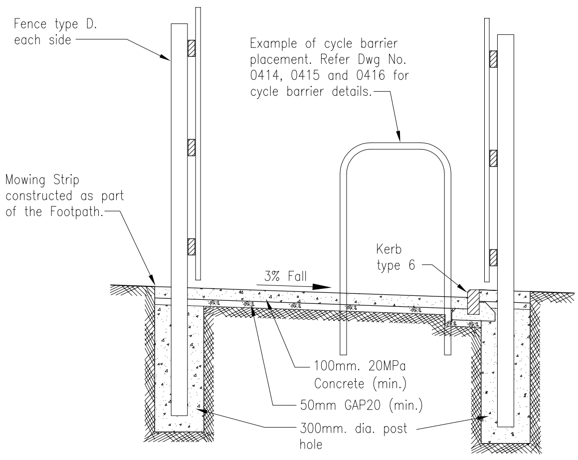
SECTIONAL ELEVATION
