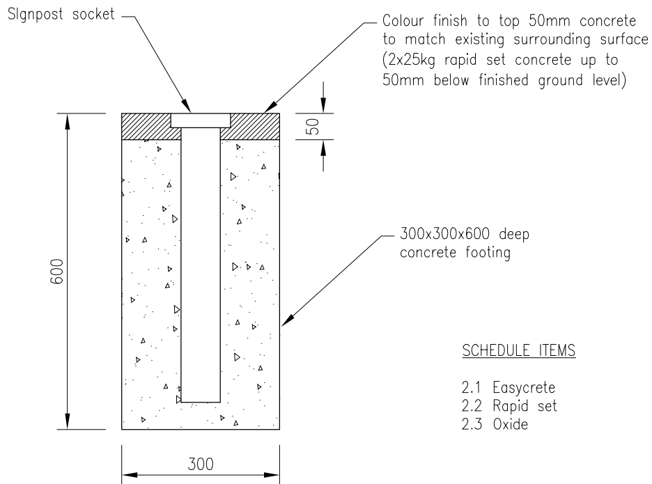
FOOTING DETAIL
