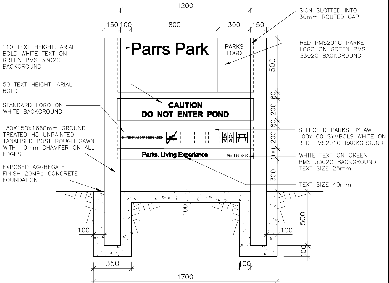
PARK SIGN WITH STORMWATER POND SAFETY SIGN
