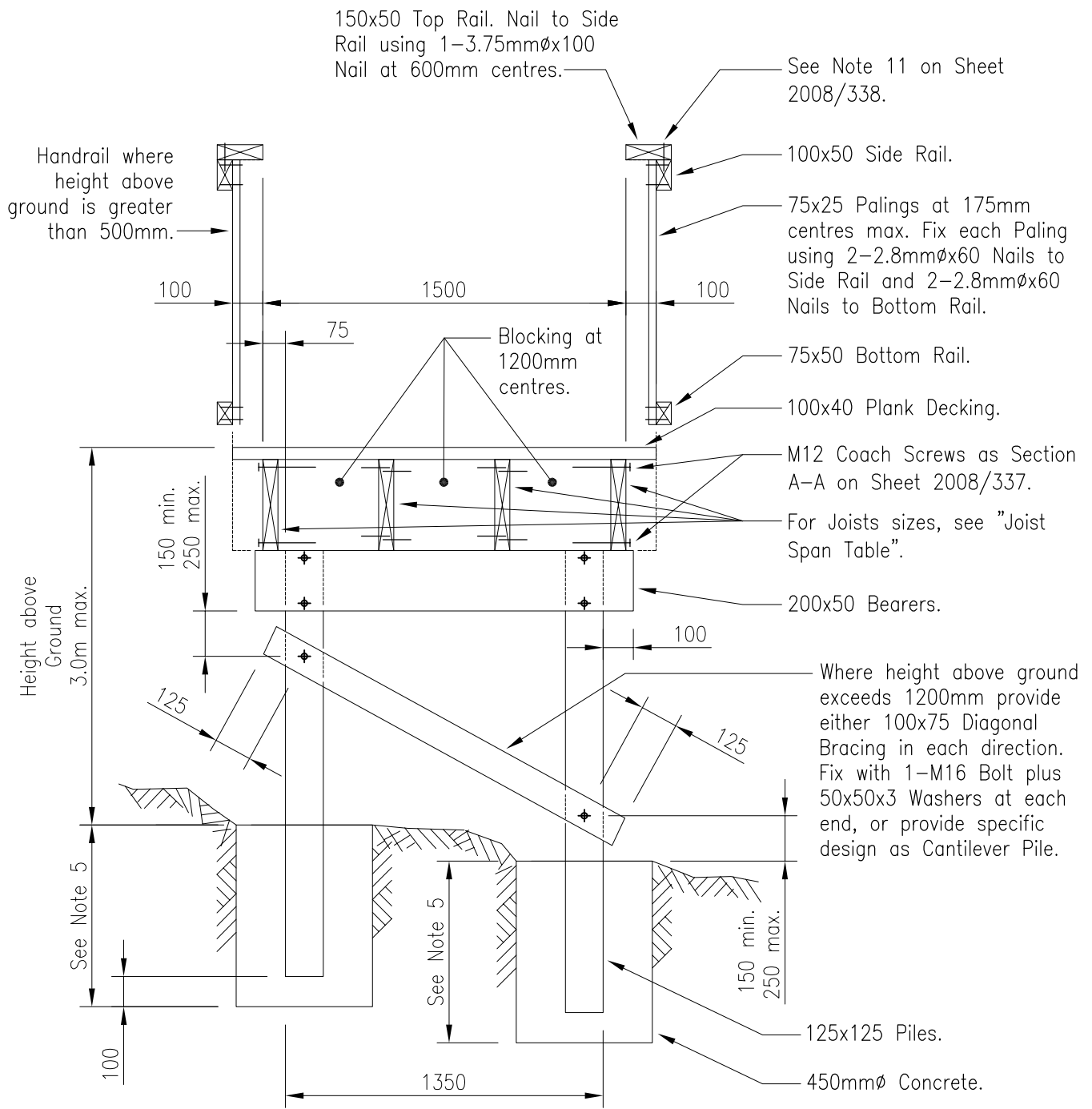
TYPICAL CROSS SECTION
