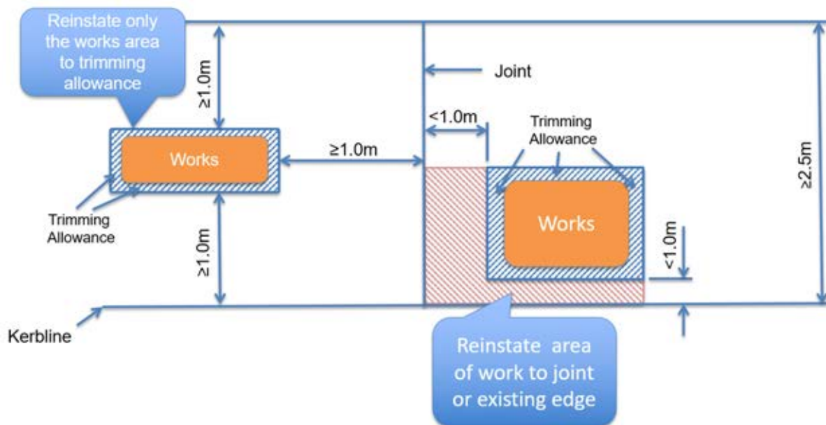
Figure 5-9: Patch reinstatement near edge or construction joint
