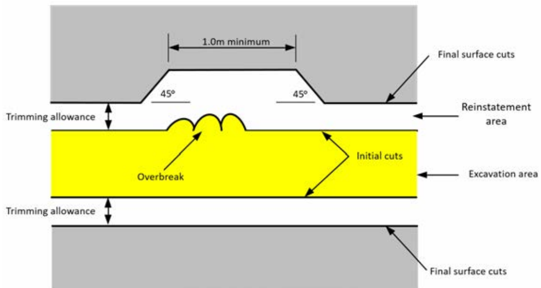
Figure 5-4: Parallel cutting of joints
