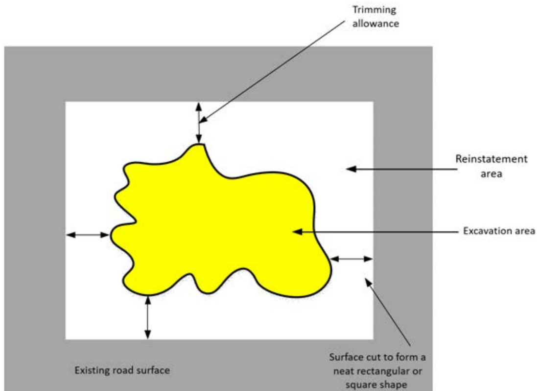
Figure 5-6: Finishing of irregular shaped excavations
