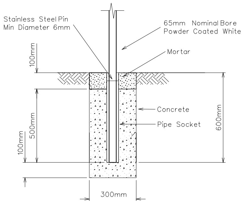
STEEL PIPE POST FOOTING DETAIL
