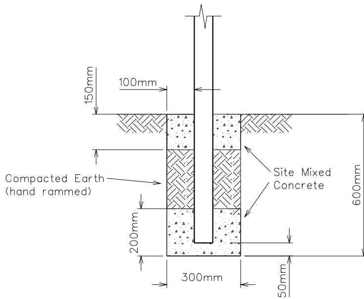
WOODEN POST FOOTING DETAIL
