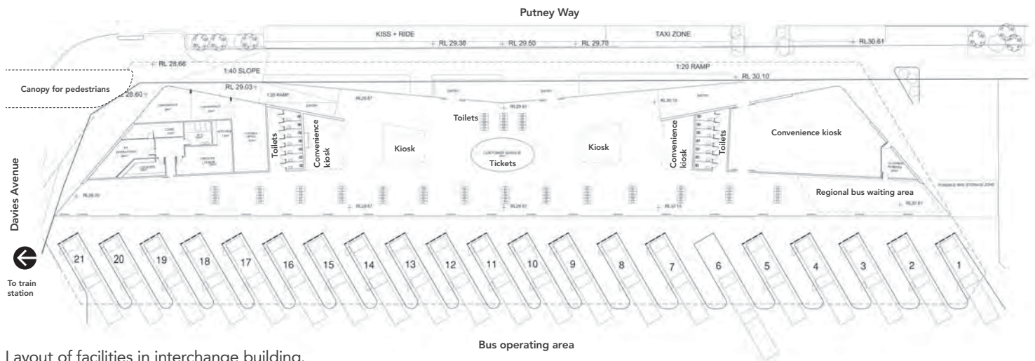
Layout of facilities in interchange building.
