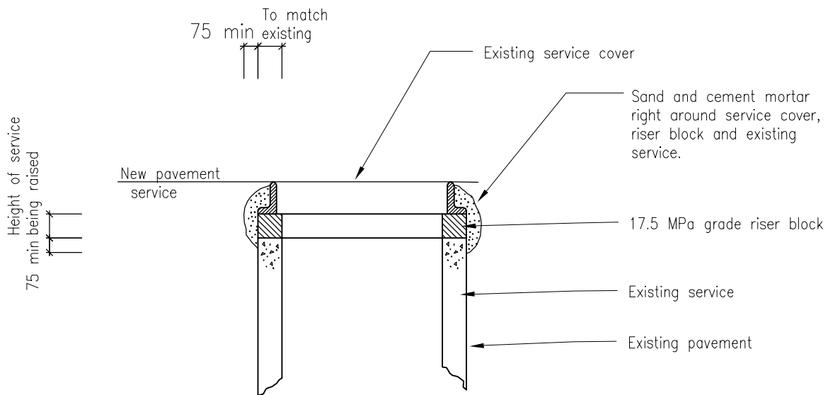
RAISED SERVICE DETAIL N.T.S
