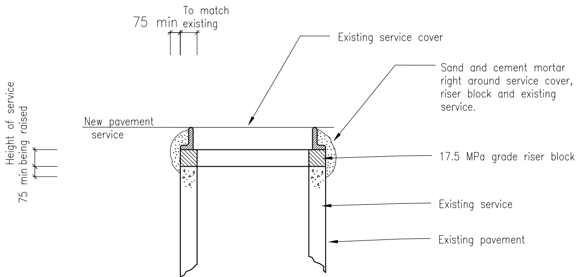
RAISED SERVICE DETAIL N.T.S
