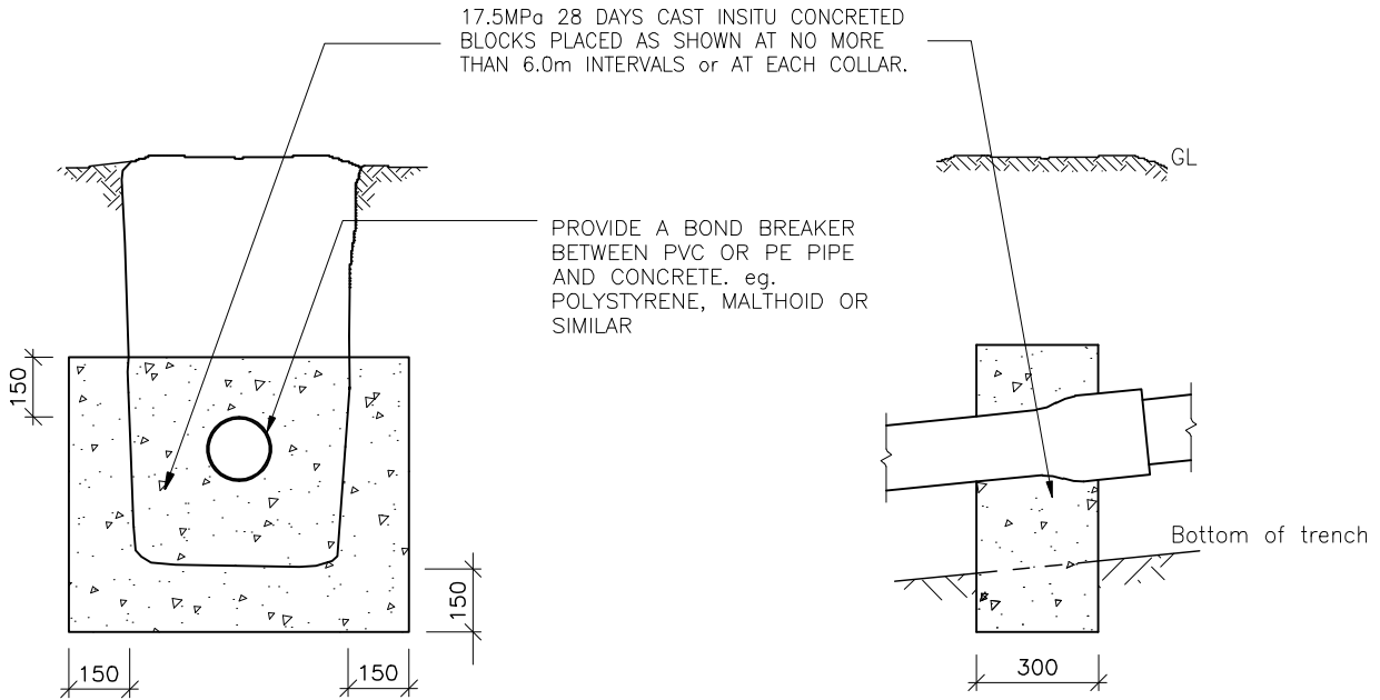
PVC, PE AND CONCRETE PIPES AT 20% OR GREATER GRADES
