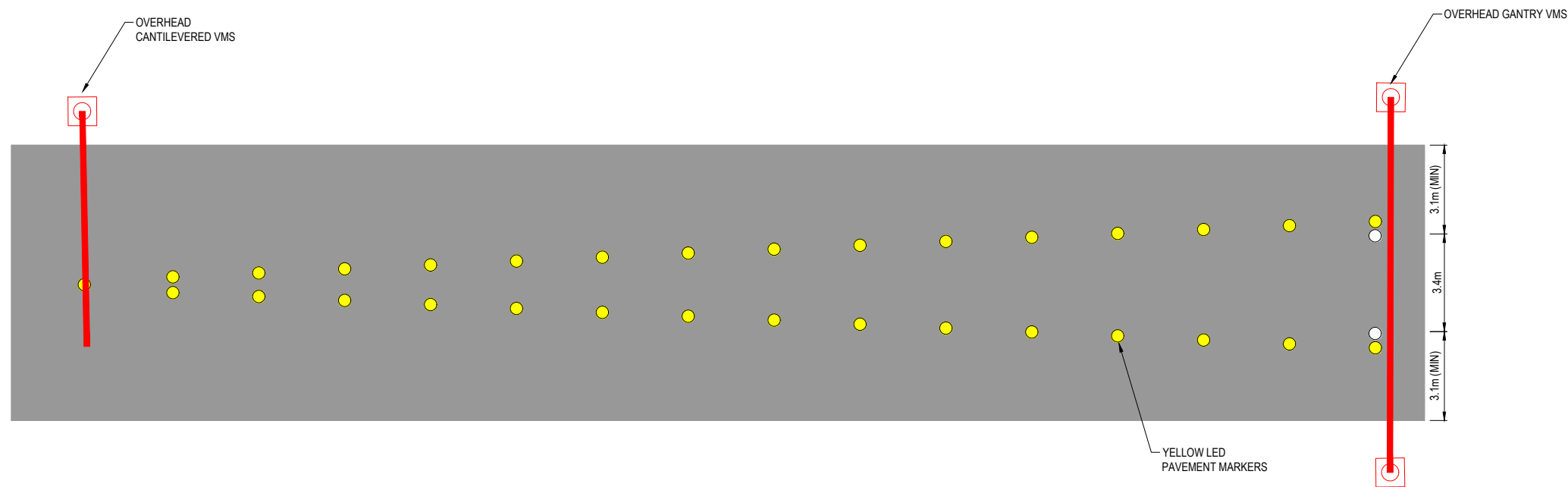
TYPICAL ENTRY LED LAYOUT N.T.S
