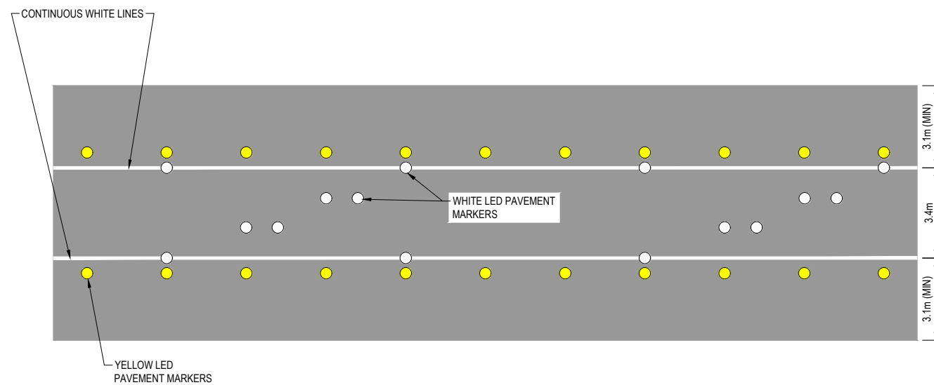
TYPICAL LED AND PAVEMENT MARKING LAYOUT N.T.S
