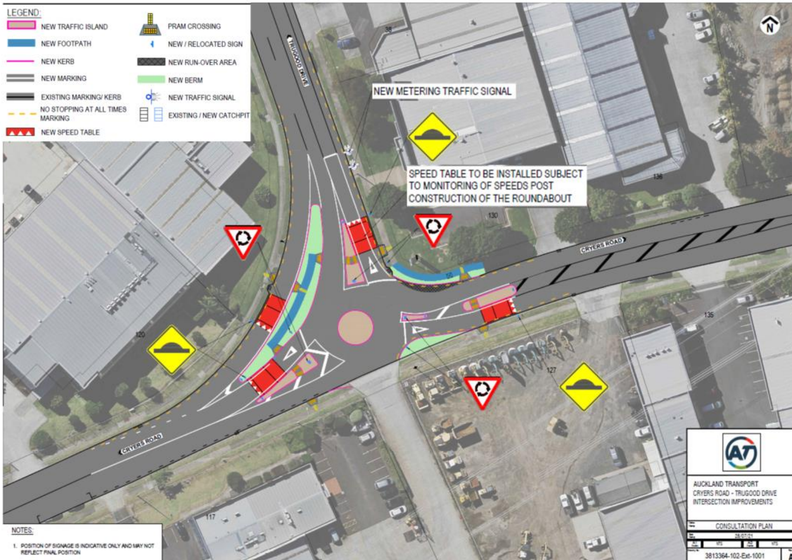
Proposed improvements for Cryers Road, Trugood Drive in Highbrook
