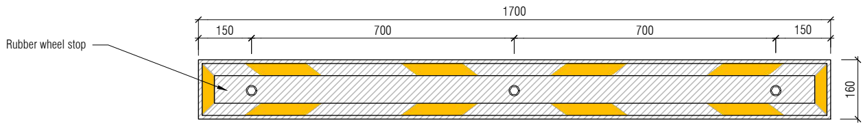
PLAN VIEW
