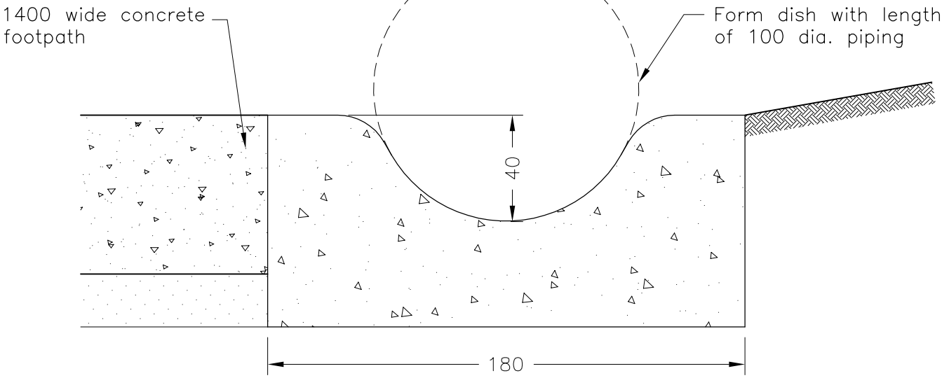
LOW LEVEL PATH
