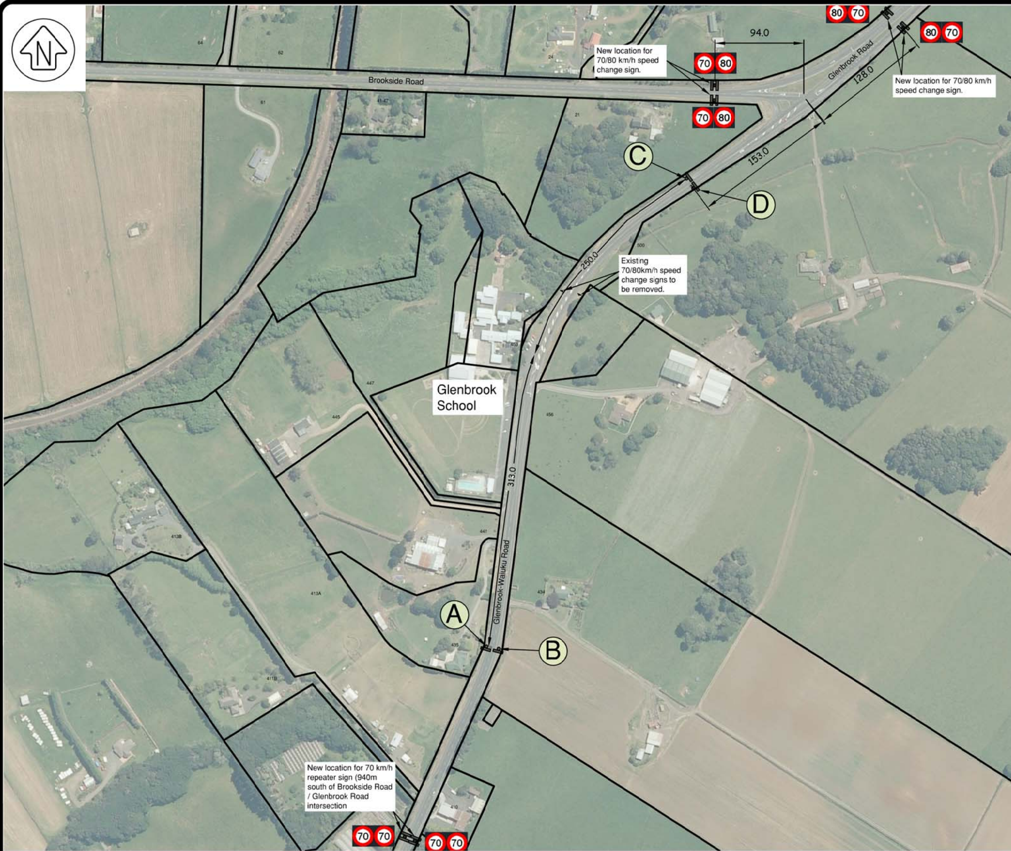
(A) (B) New "40 km/h Advisory" sign located 716m south of Glenbrook Road / Brookside Road intersection.
