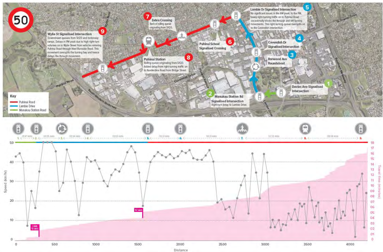
Figure 6-1: Travel Time surveys AM Peak: Westbound
