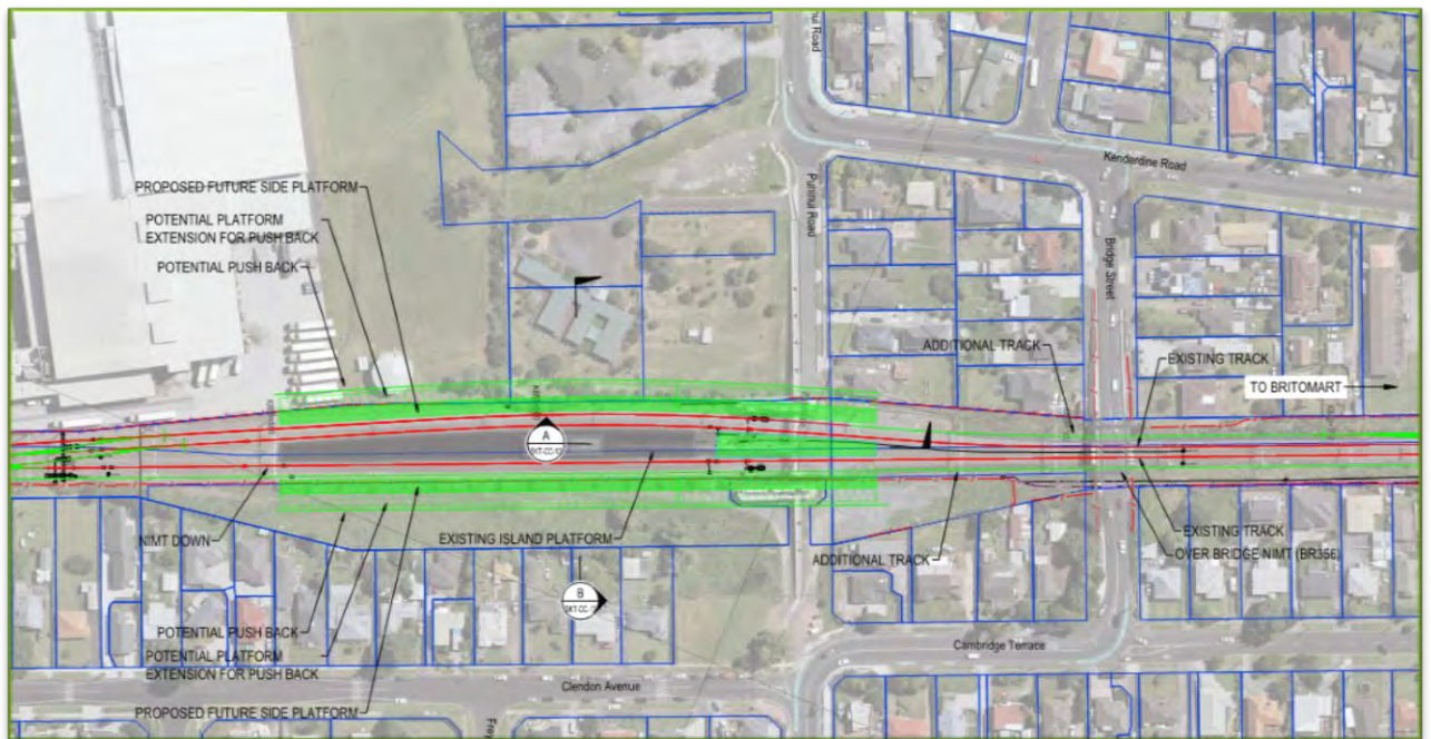
Figure 4-4: Layout of future proofing to rail corridor
