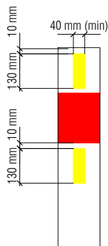
TYPE C: YELLOW RETROREFLECTOR
