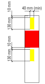
TYPE C: YELLOW RETROREFLECTOR
