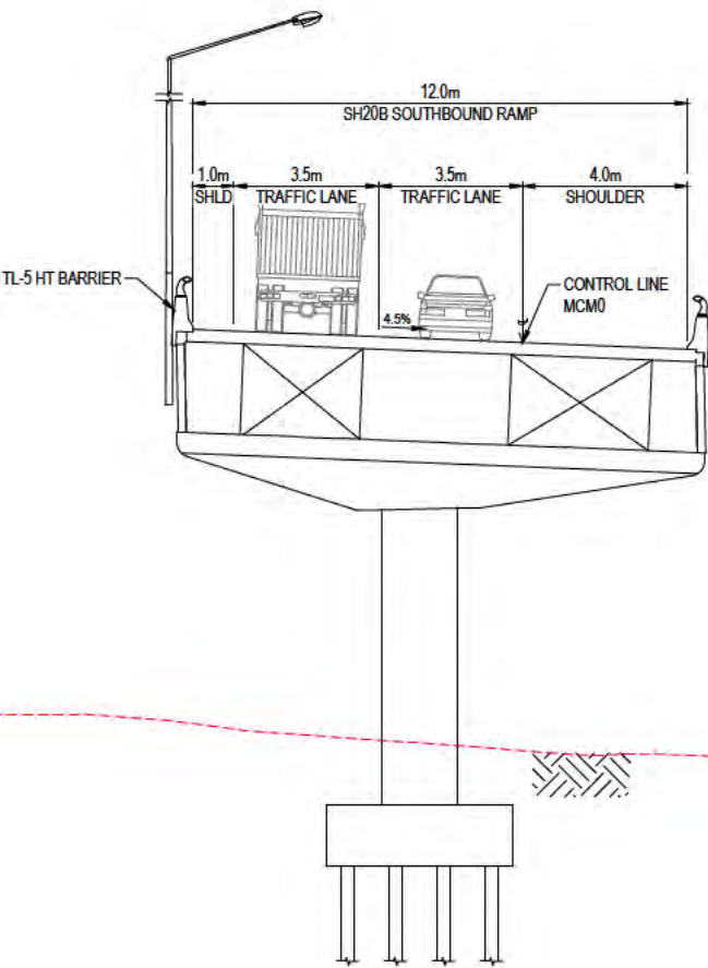
SECTION R CH410 (MCM0) RR-1112 SH20B SOUTHBOUND RAMP BRIDGE TYPICAL CROSS SECTION
