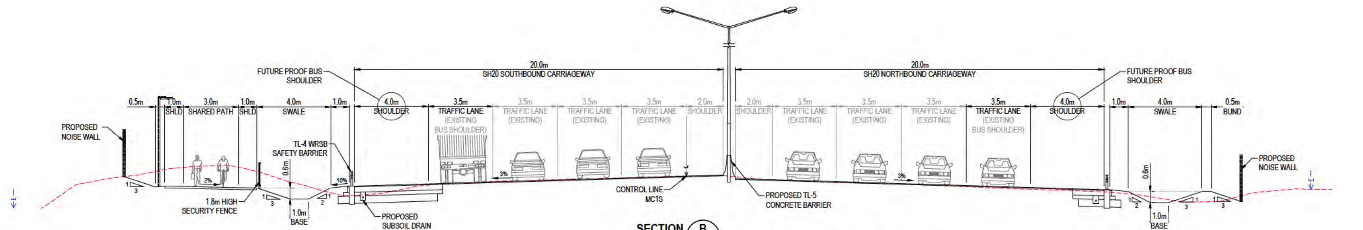
SECTION B CH12,960 (MC1S) RR-1102 SH20 TYPICAL CROSS SECTION WITH SWALES
