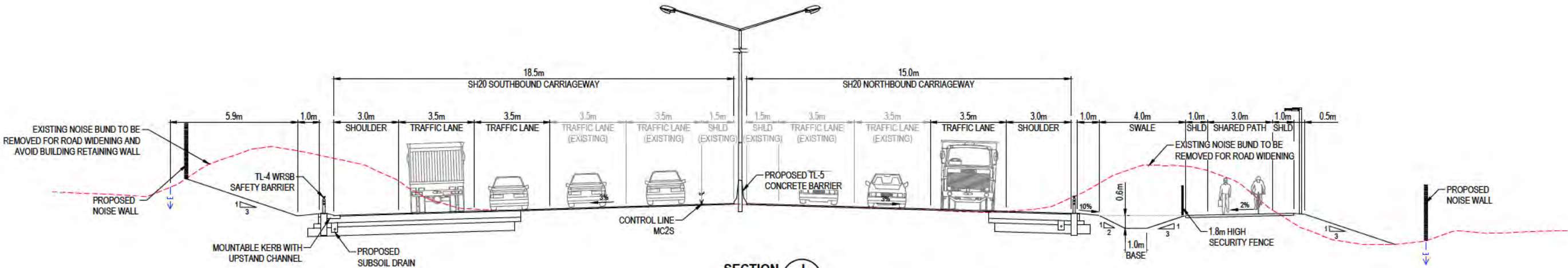
SECTION J SH20 TYPICAL CROSS SECTION WITH SWALES
