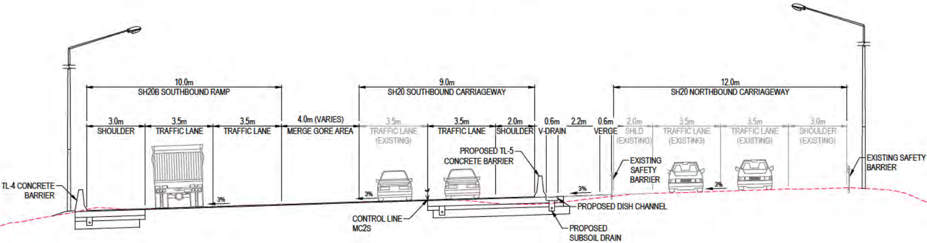
SECTION S CH6,300 (MC2S) RR-1113 SH20 TYPICAL CROSS SECTION WITH MEDIAN WIDENING ON SUPERELEVATION
