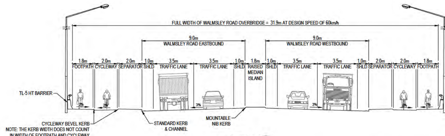
SECTION C RR-1103 SH20 WALMSLEY ROAD OVERBRIDGE TYPICAL CROSS SECTION
