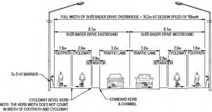
SECTION H SH20 BADER DRIVE OVERBRIDGE TYPICAL CROSS SECTION
